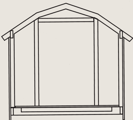
FRONT TRUSS
