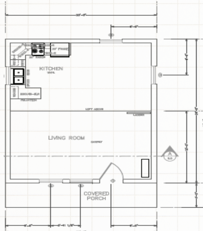
Lower Level Floorplan
