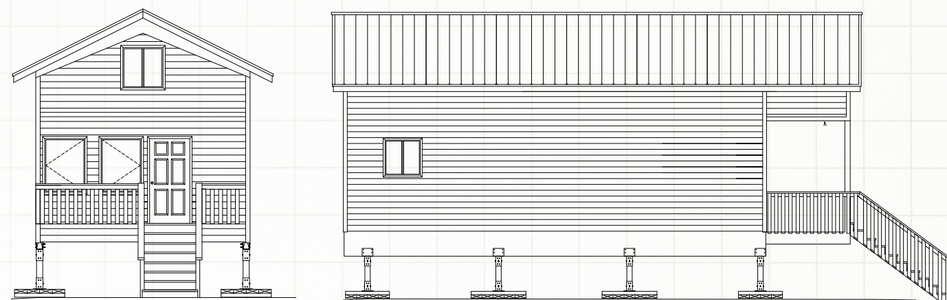
Front Elevation
